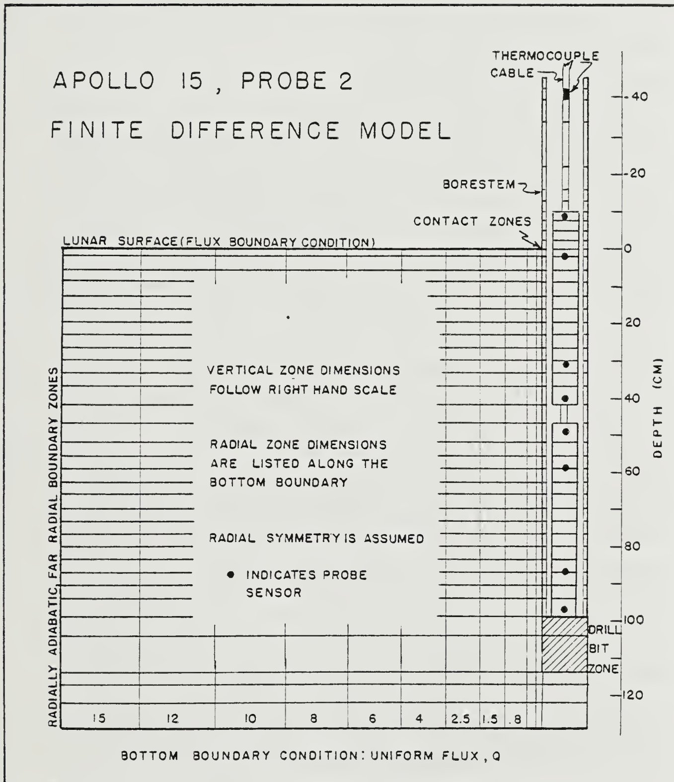
Schematic of Apollo 15 probe 2 numerical model
